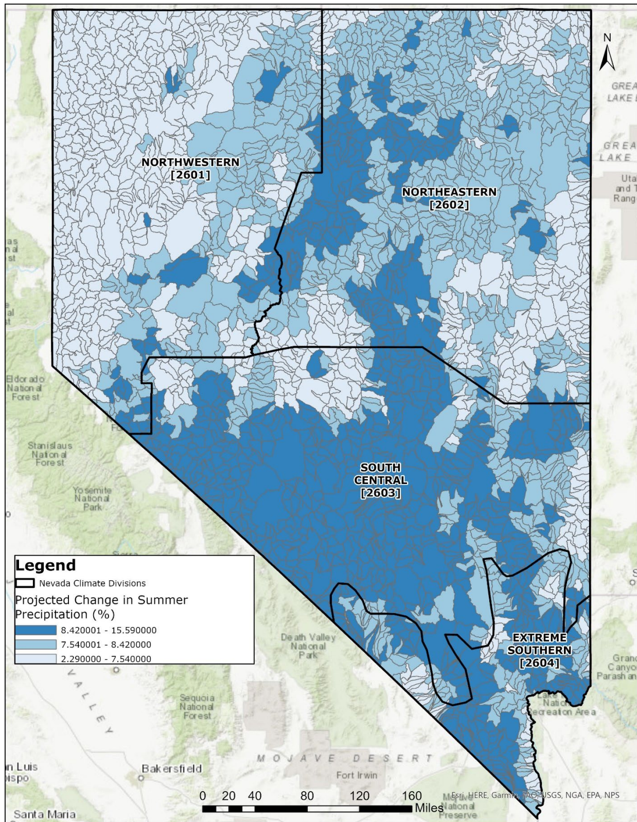
Figure 7: Projected Change in Summer Precipitation (%)
