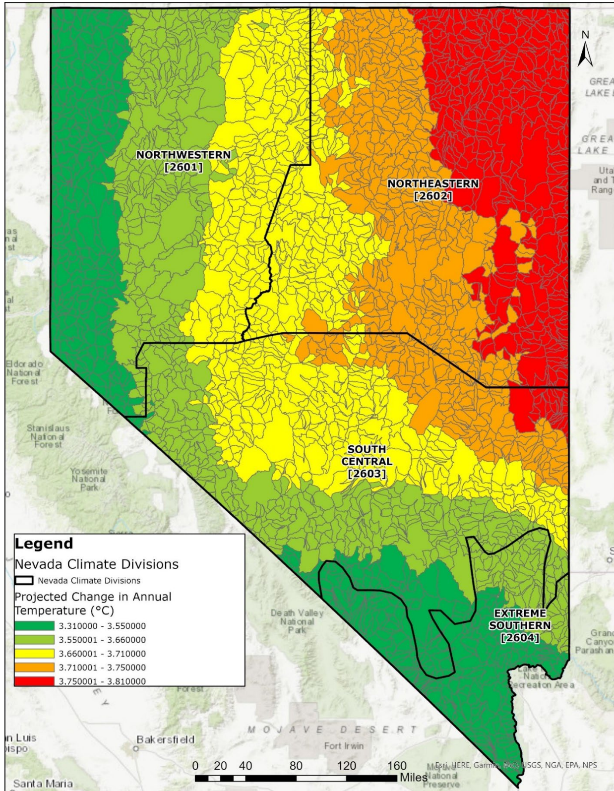
Figure 3: Projected Change in Annual Temperature (°C)
