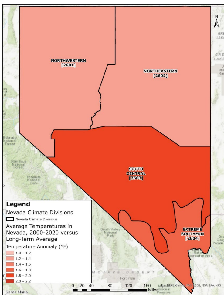
Figure 1: Average Temperatures in Nevada, 2000-2020 versus Long-Term Average
