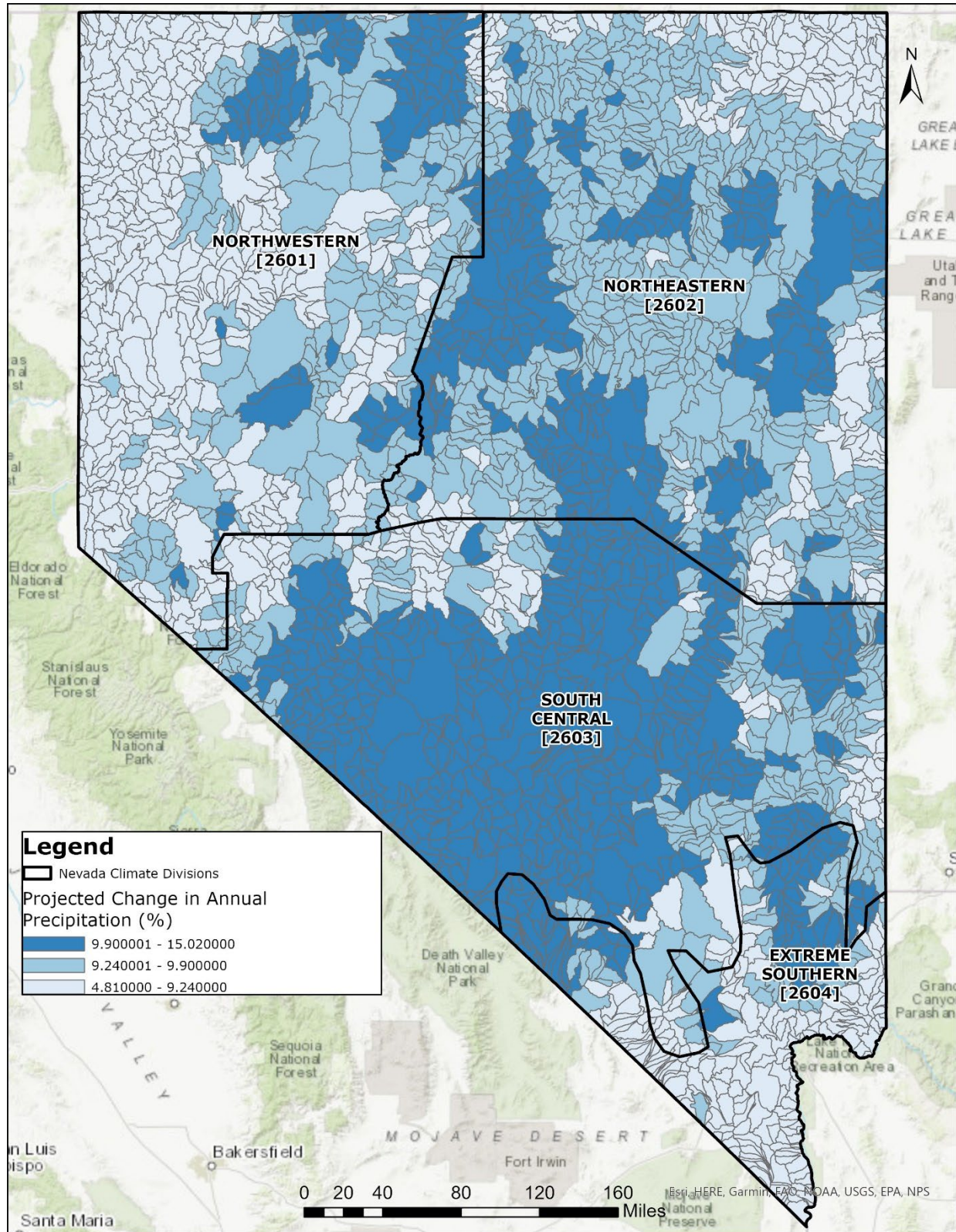
Figure 6: Projected Change in Annual Precipitation (%)
