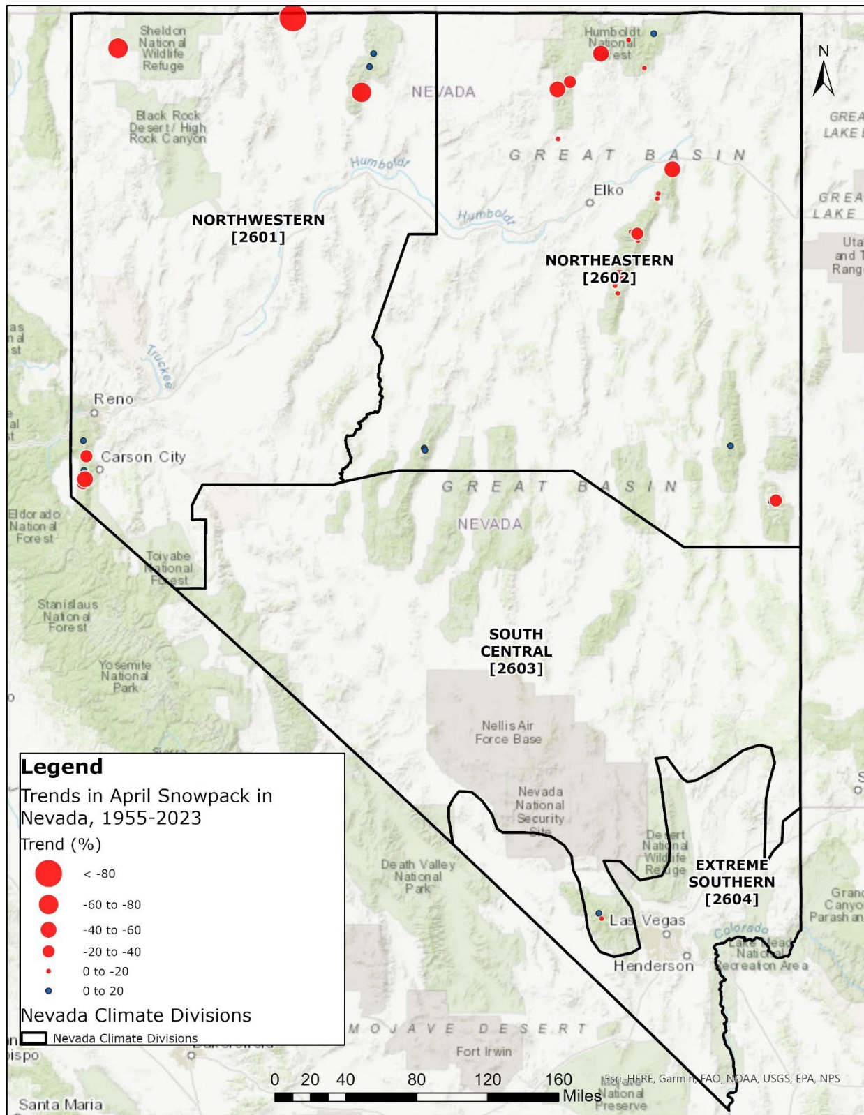
Figure 8: Trends in April Snowpack in Nevada, 1955-2023
