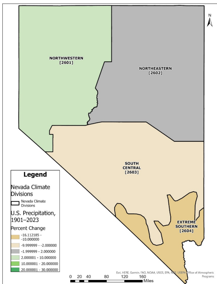
Figure 5: Percent Change in Total Annual Precipitation in Nevada, 1901-2023
