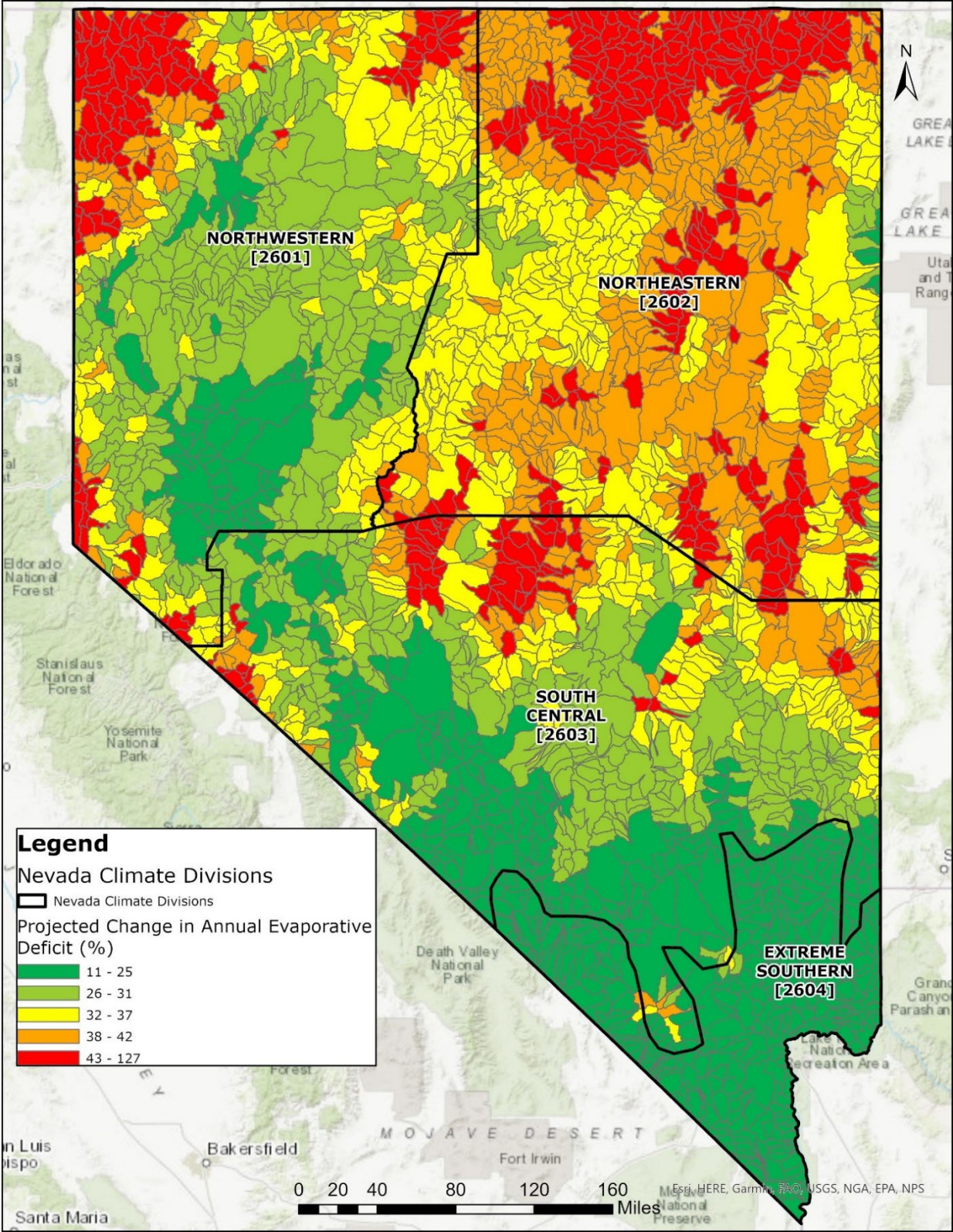
Figure 13: Projected Change in Annual Evaporative Deficit (%)
