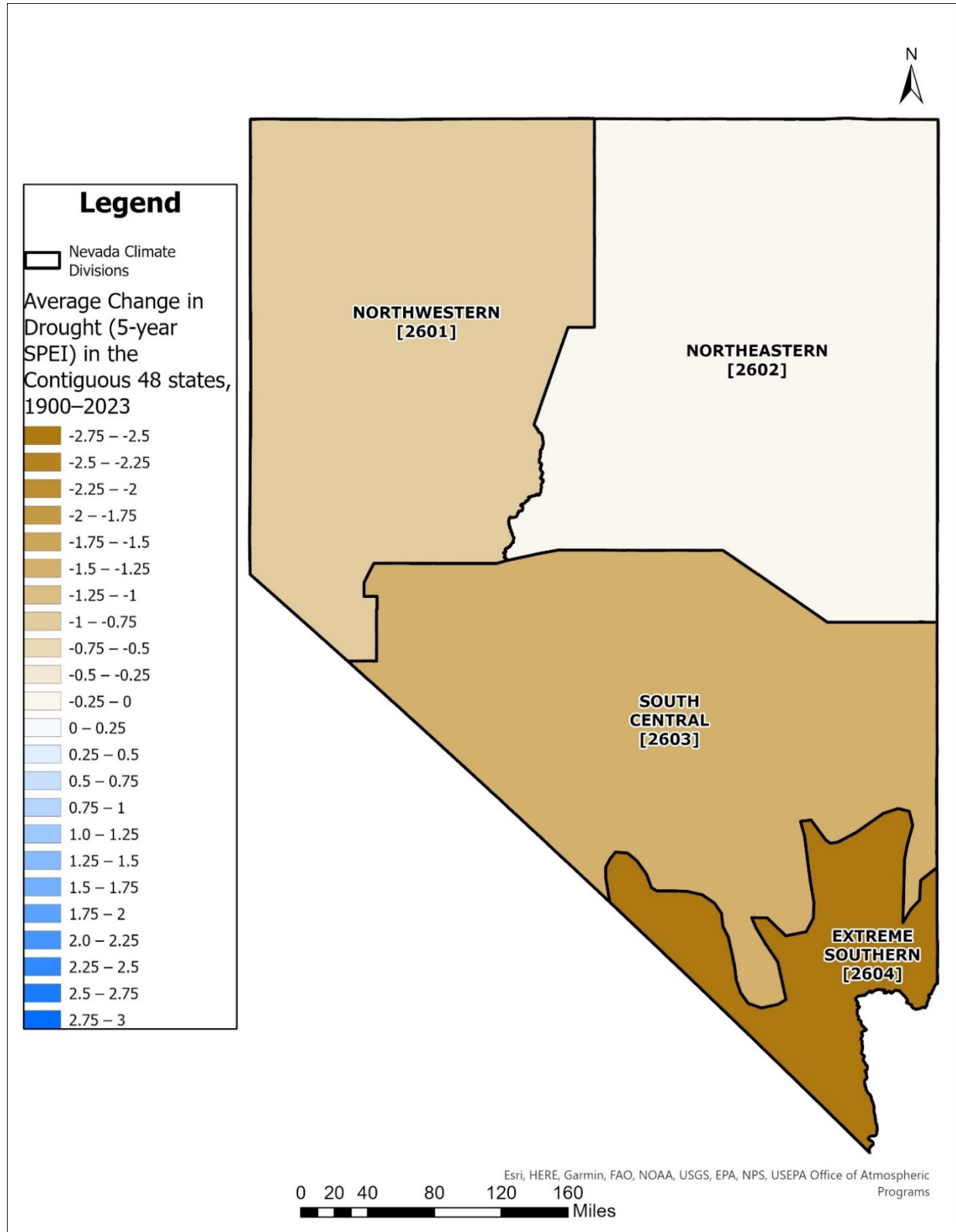
Figure 12: Average Change in Drought (5-year SPEI) in Nevada, 1900-2023
