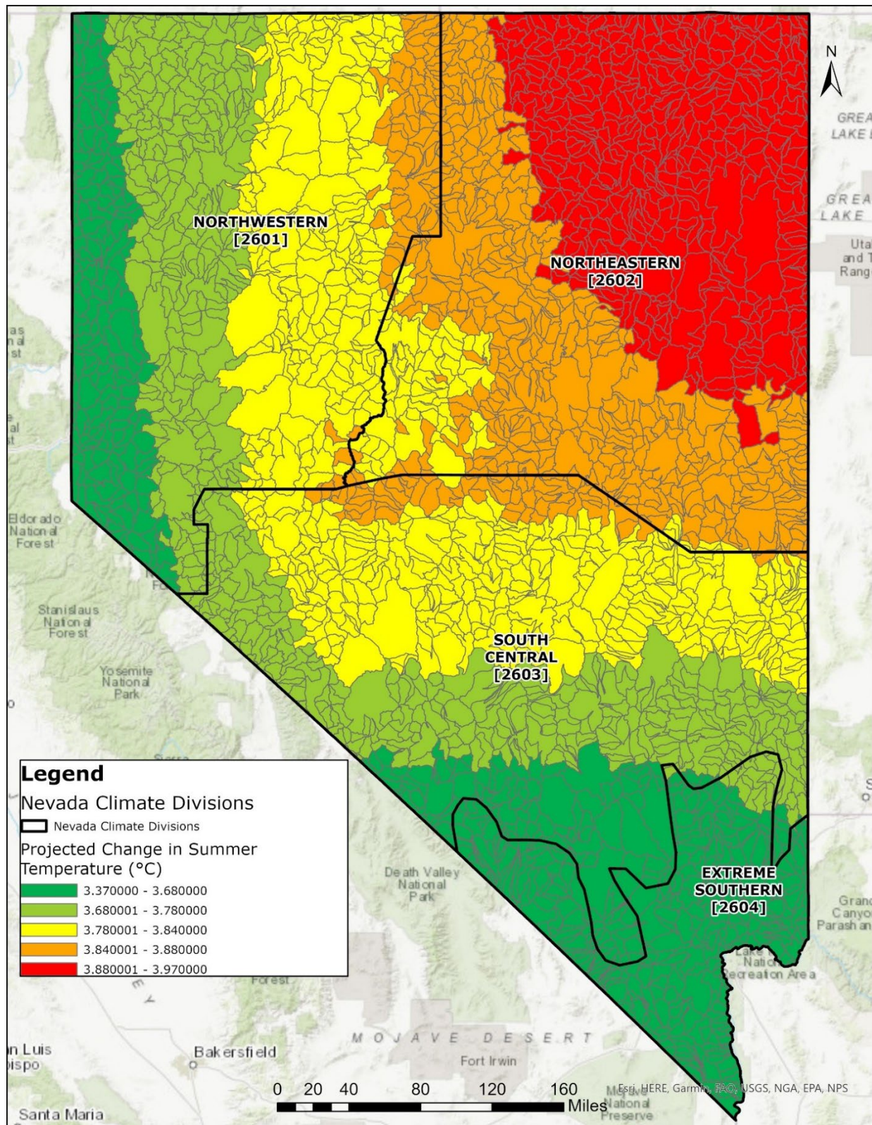
Figure 4: Projected Change in Summer Temperature (°C)
