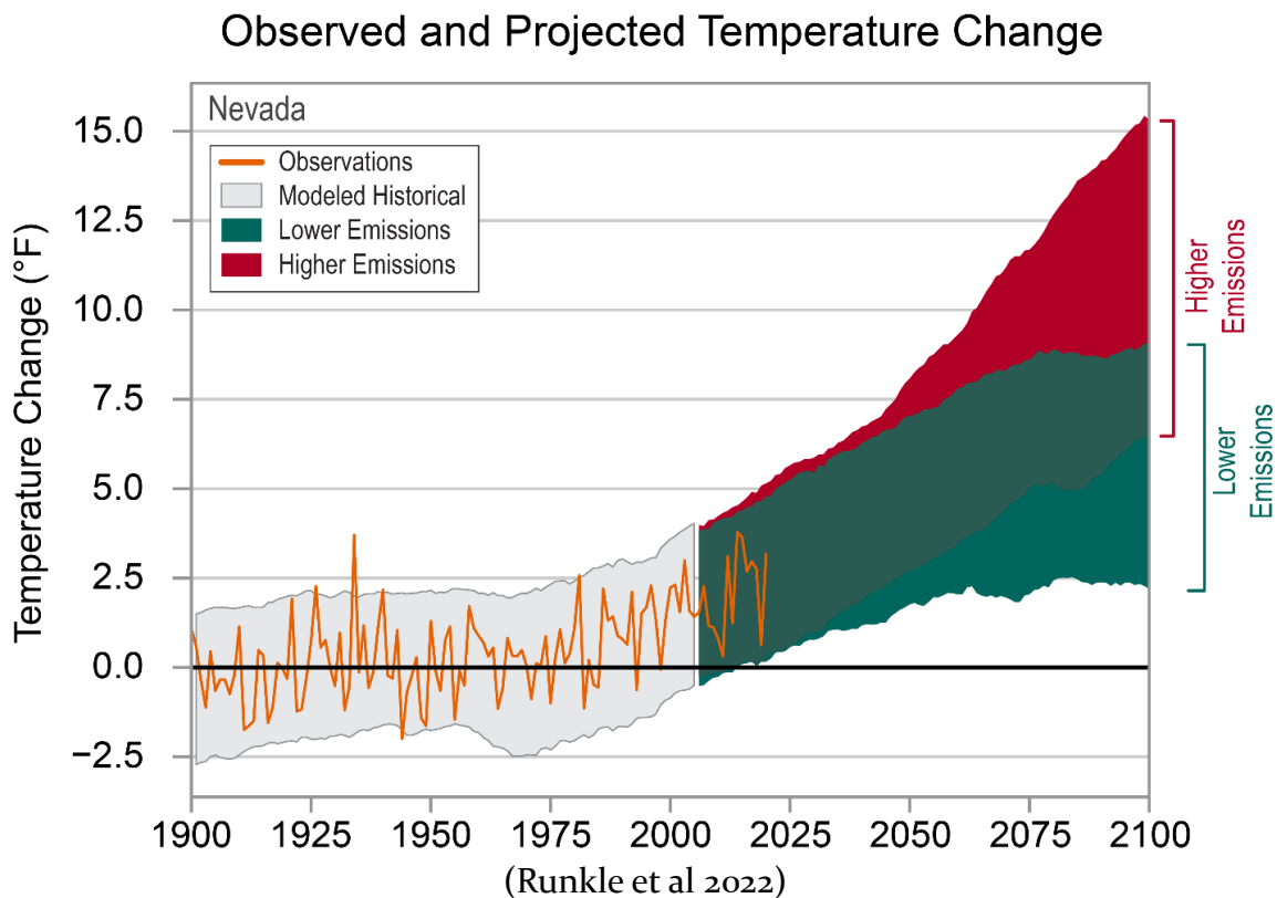
Figure 2: Observed and Projected Temperature Change in Nevada
