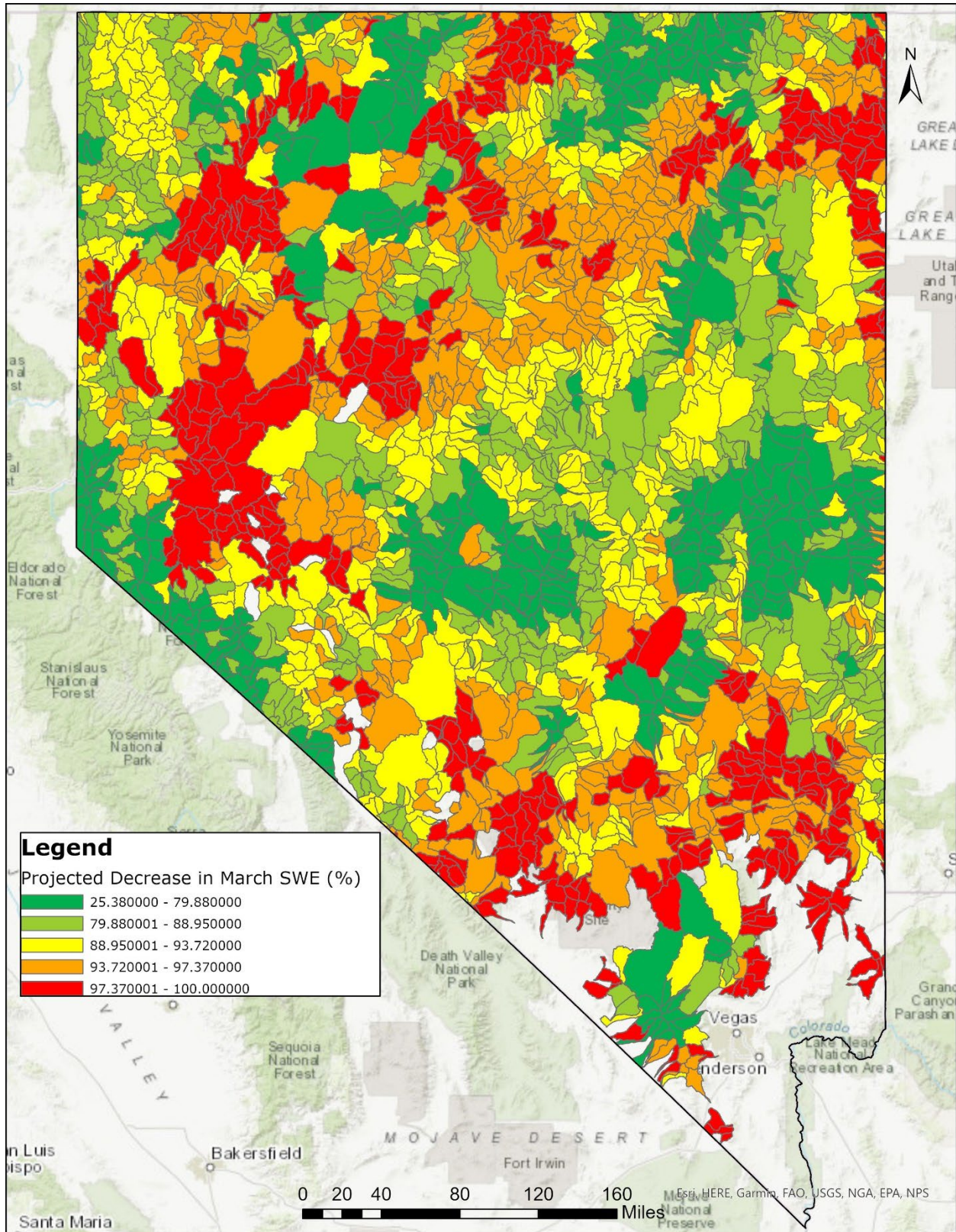
Figure 9: Projected Decrease in March Snow Water Equivalence (%)
