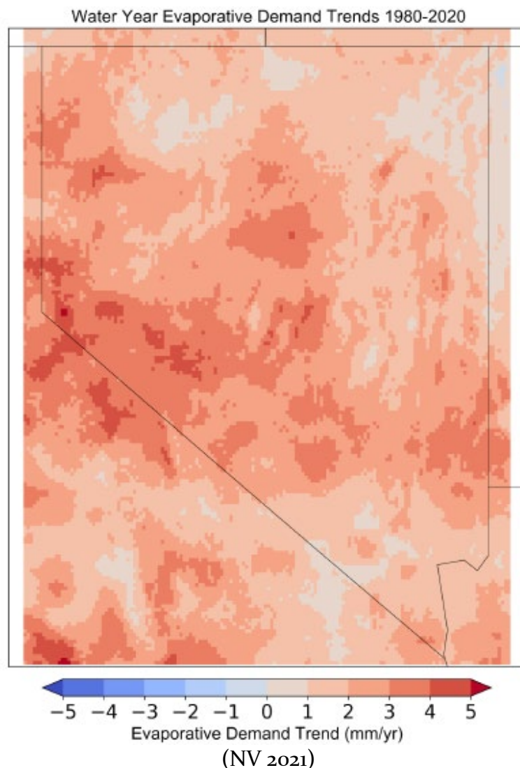
Figure 11: Observed trends total evaporative demand for the period 1980–2020
