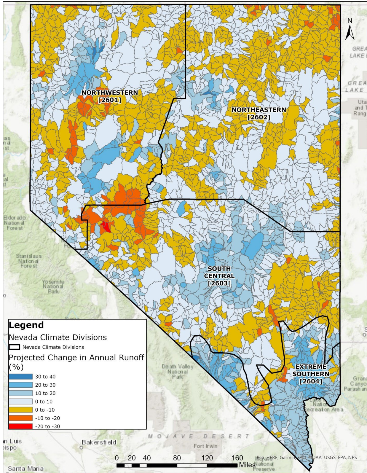
Figure 10: Projected Change in Annual Runoff (%)
