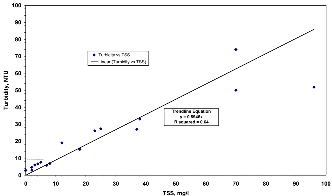
Figure 11. Turbidity vs. TSS - Bryant Creek at Doud Springs, Nevada (at BCU)
