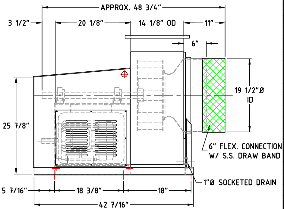
FAN DISCHARGES - VIEWED FROM DRIVE SIDE
