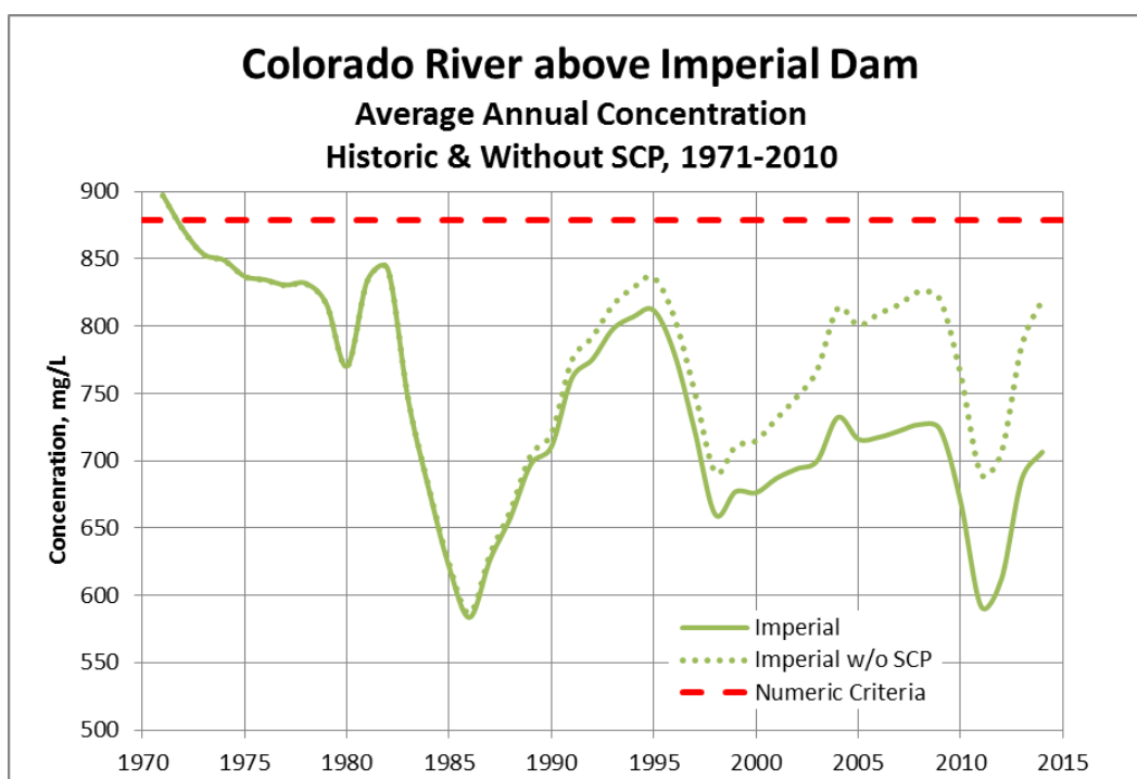
Figure 5 – Salinity Control Program Impact at Imperial Dam
