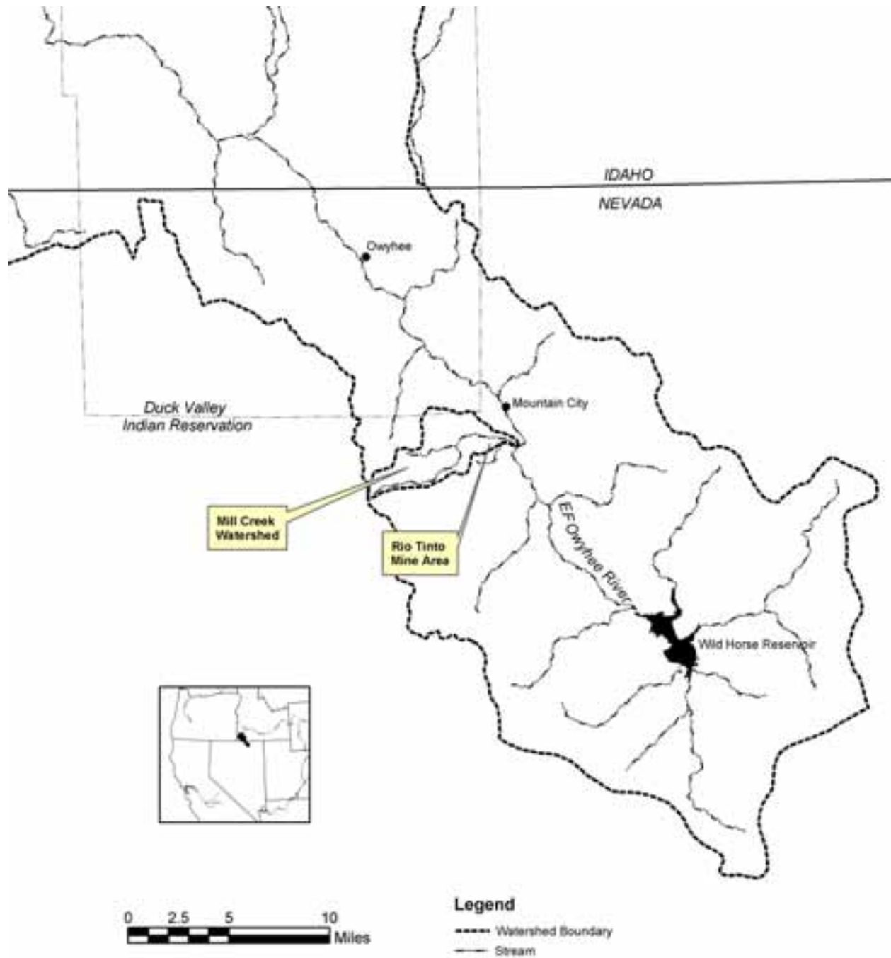
Figure 1. East Fork Owyhee River and Mill Creek Location Map
