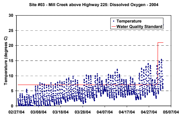
Figure 6. Temperature Data Collected on Mill Creek by Shoshone-Paiute Tribes and EPA
