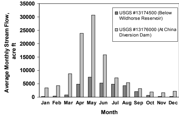
Figure 4. Average Monthly Stream Flow at Selected Sites on East Fork Owyhee River
