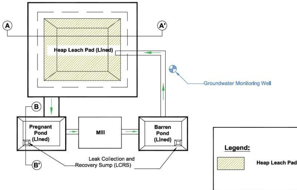
Figure 1: Top view of an idealized heap leach pad with associated process ponds.
