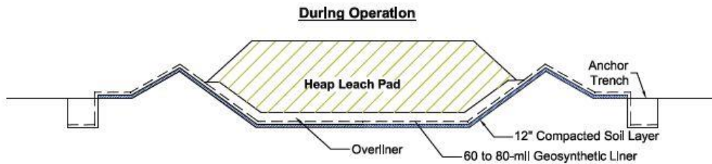
Figure 2: Side view of an idealized heap leach pad showing the liner system at the bottom. Current design criteria requires installation of a system to detect leakage from the heap leach pad, typically a network of monitoring wells.
