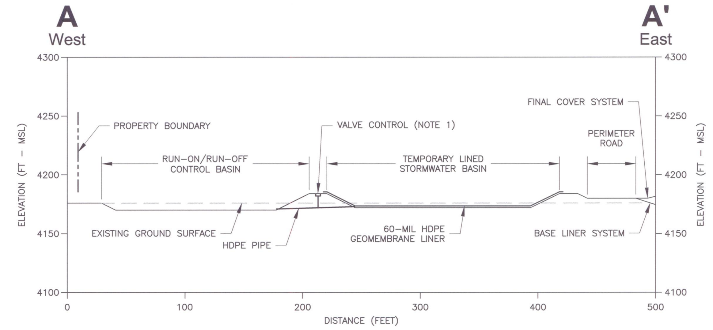
A 3E3E BASIN PROFILE SECTION 50 0 50 HORI. & VERT. SCALE FEET
